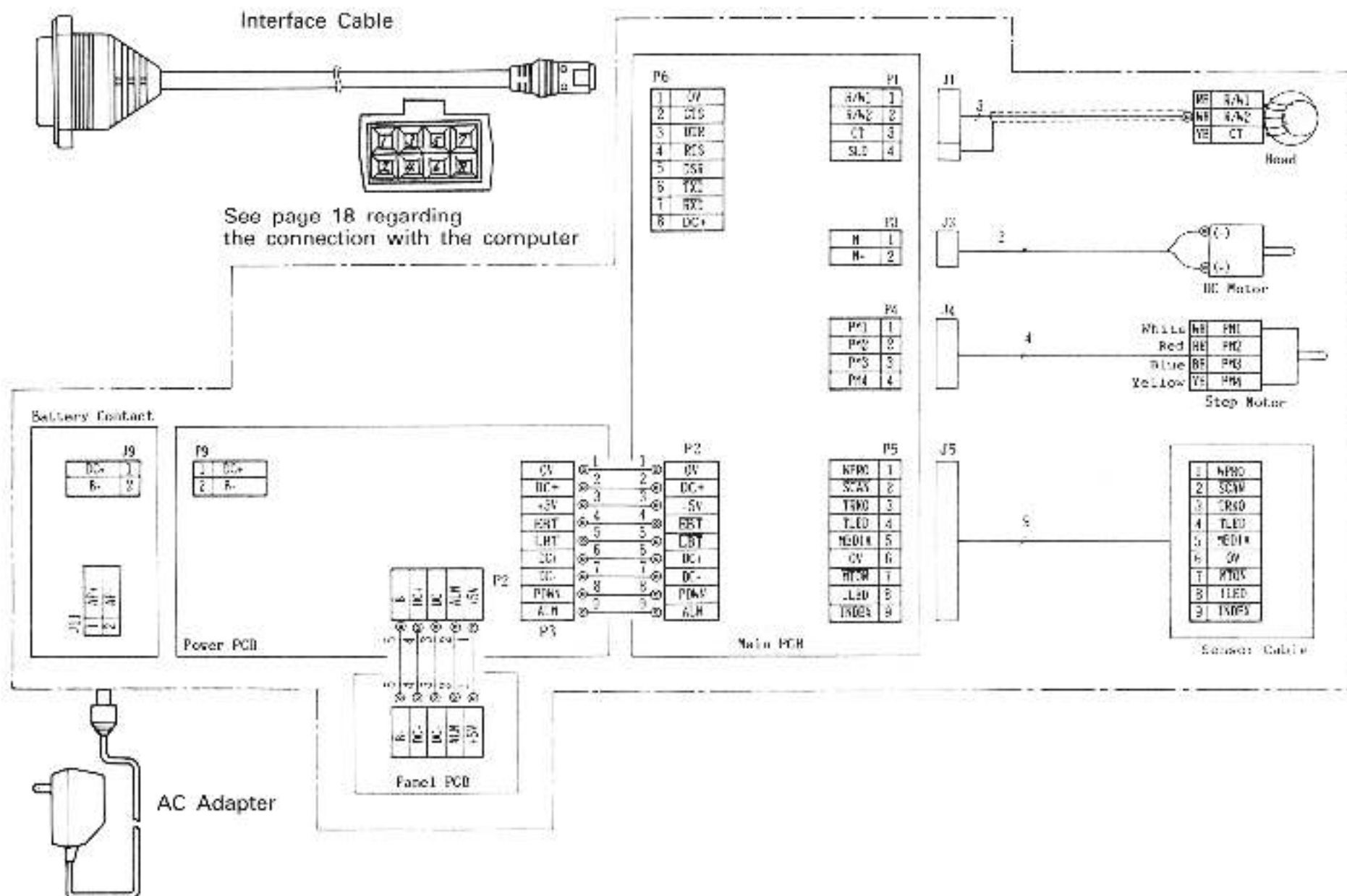
Fig. 6-1 Connection Diagram
