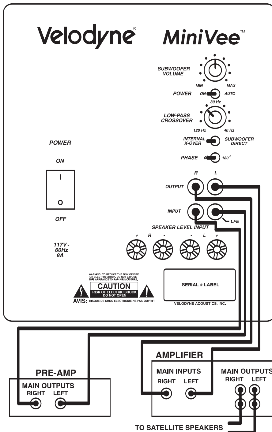
Figure 2. Installation Using Stereo Line-Level Inputs
