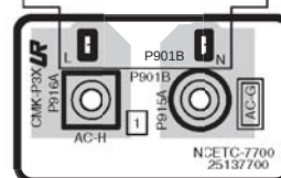
AC INLET PC BOARD (NAETC-7700) Except 120V and Australian models
