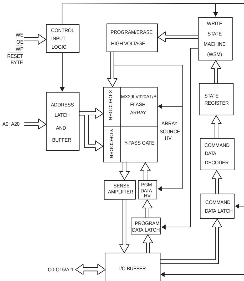
BLOCK DIAGRAM
