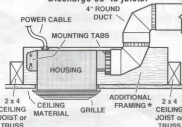
HOUSING MOUNTED TO 2x4 TRUSS
