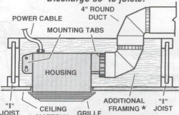
HOUSING MOUNTED TO "1" JOIST
