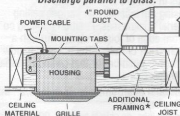
HOUSING MOUNTED TO ADDITIONAL FRAMING
