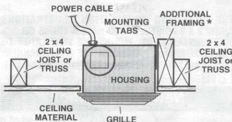
HOUSING MOUNTED TO 2x4 TRUSS
