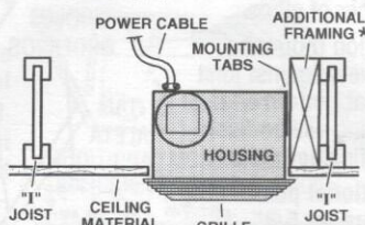
HOUSING MOUNTED TO "1" JOIST
