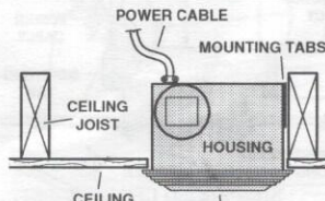
HOUSING MOUNTED DIRECTLY TO JOIST 2x6 (or larger)
