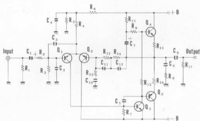
Fig. 6 Circuit Diagram of Equalizer Amplifier
