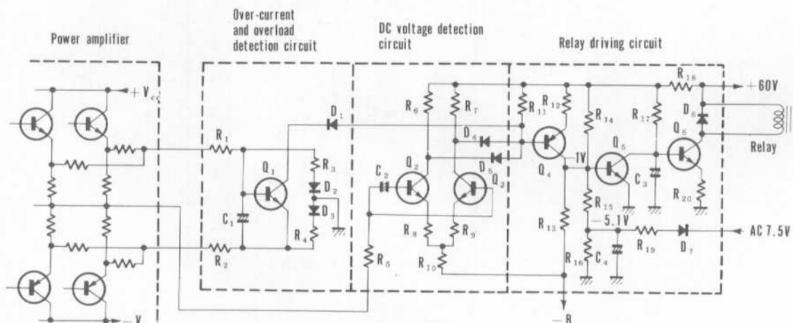
Fig. 15 Protection Circuit
