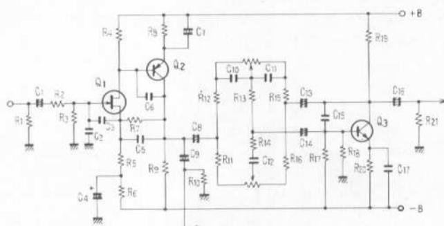
Fig. 8 Tone Control Circuit
