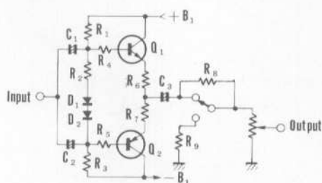
Fig. 7 Input Buffer Amplifier
